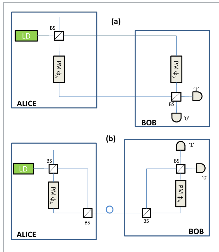
■ Figure 3. Layout of a QKD system using Phase coding for (a) single Mach-Zehnder configuration and (b) unbalanced Mach-Zehnder configuration.
