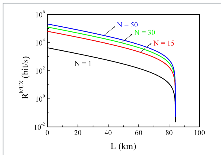
■ Figure 7. Overall useful key rate values versus the optical fiber link length in Km, obtained for the three frequency plan ( N=15 , N=30 and N=50 ) systems and for the case of a frequency coded ( N=1 ) system when the index modulation is m=2\% .
