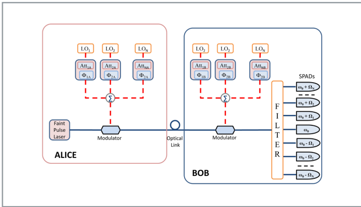
■ Figure 5. SCM-QKD system layout (electrical signal is in dashed line, optical signal in solid line). SPAD: Single Photon Avalanche Detector.
