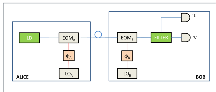
■ Figure 4. Layout of a Frequency Coded QKD transmission system.
