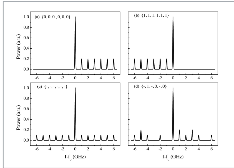
■ Figure 6. Simulated power spectra for perfect matching between the basis employed by Alice and Bob for each subcarrier and Alice is sending (a) the sequence 000000 and (b) the sequence 111111. In case (c), Bob makes the incorrect basis decision for all the subcarriers and in case (d), Bob makes the correct basis decision for subcarriers f_1 , f_3 and f_5 . For cases (c) and (d), the sequence is 011010.
