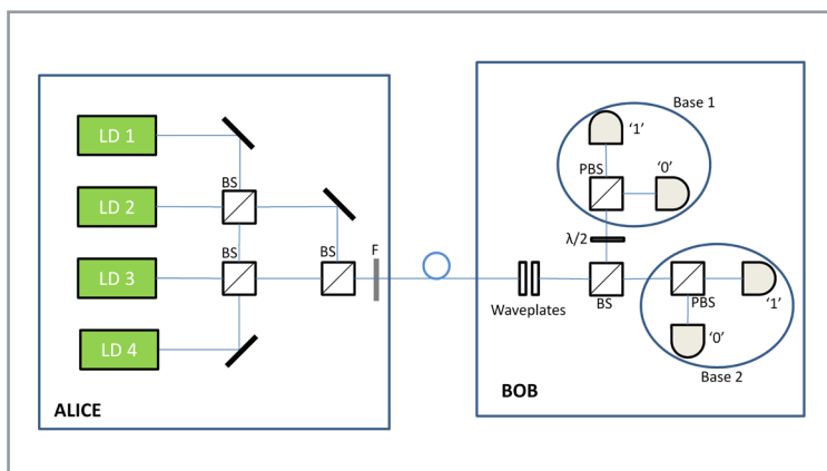
■ Figure 2. Layout of a typical BB84 QKD system based on Polarization encoding.
