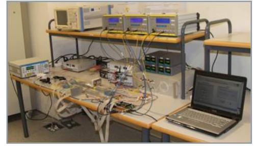
■ Figure 9. Experimental setup assembled in the laboratory to test the feasibility of a two channel sub-carrier multiplexed quantum key distribution system
