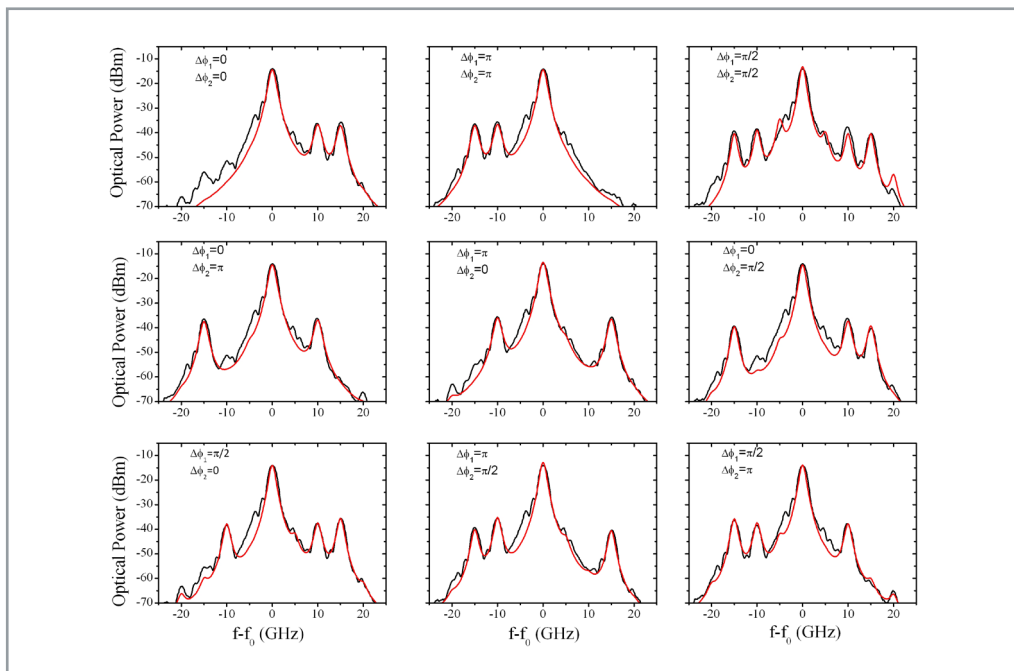
■ Figure 11. Experimental (black line) and theoretical (red line) results and for a two subcarrier SCM-QKD system for different phase match values between Alice and Bob. Subcarrier frequencies are 10 and 15 GHz respectively.
