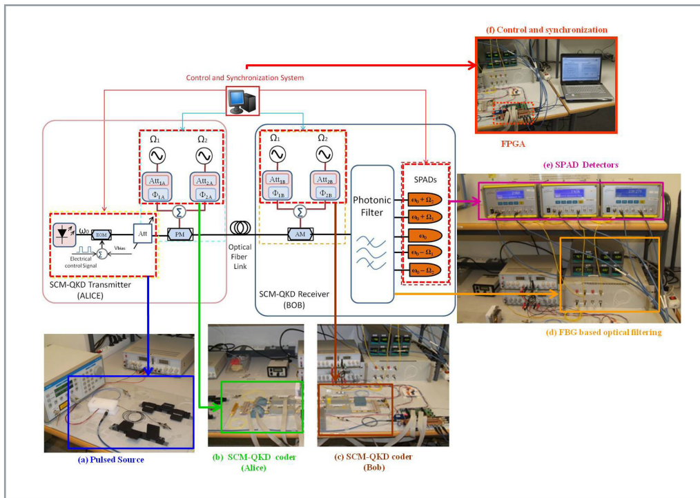
■ Figure 10. Experimental setup assembled in the laboratory to test the feasibility of a two channel subcarrier multiplexed quantum key distribution system
